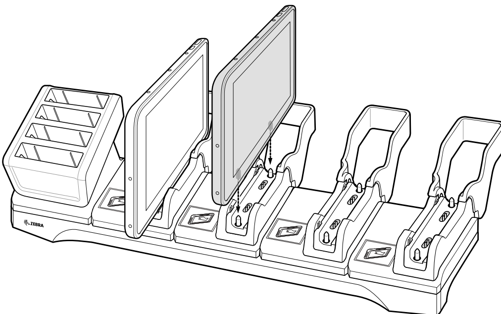
Figure 106 Insert ET5X without Rugged Frame into Slot
