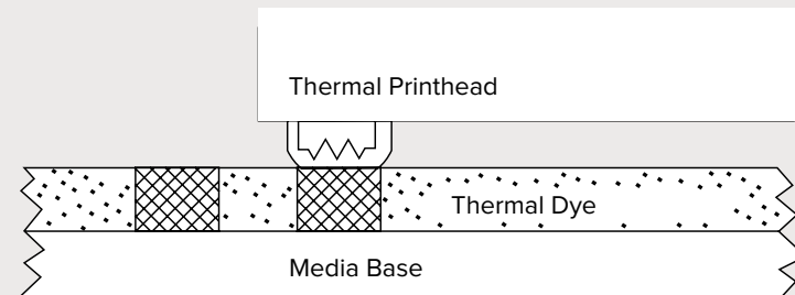
Figure 5. Direct Thermal Printing
