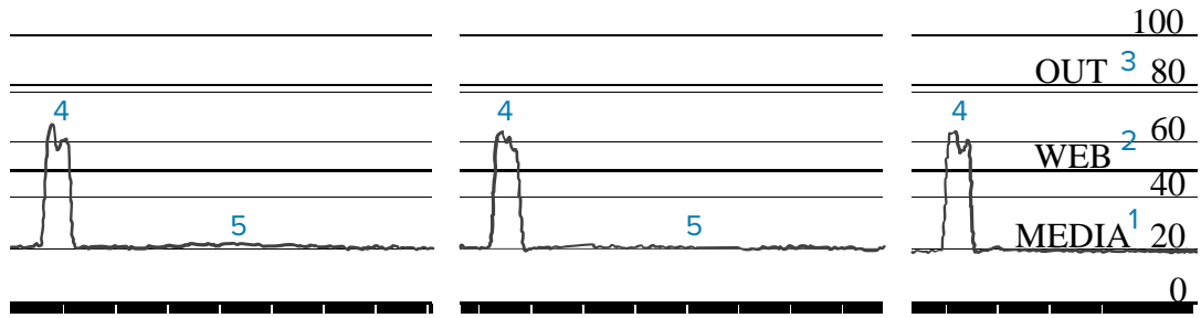
图 10 Media Sensor Profile (Black Mark Media)
