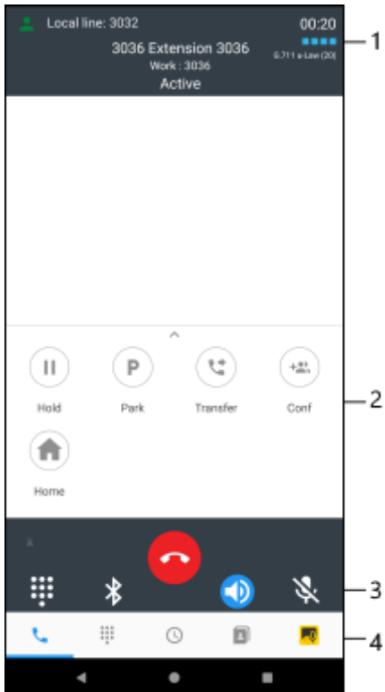
Figure 15 In-Call Dashboard
