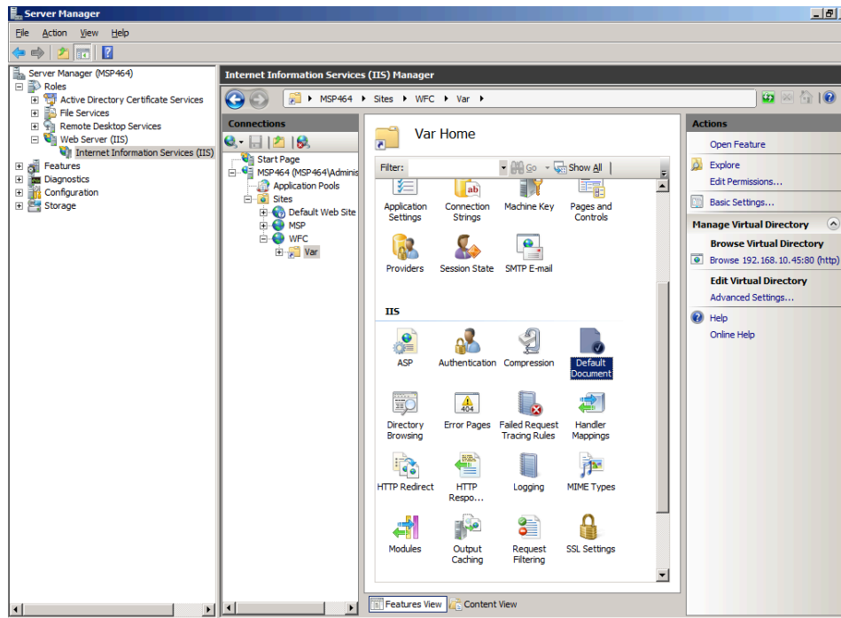
Figure 5 Server Manager
