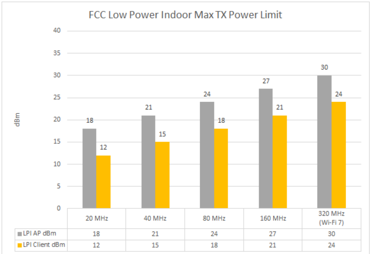
Figure 9 FCC Low Power Indoor Max TX Power Limit
