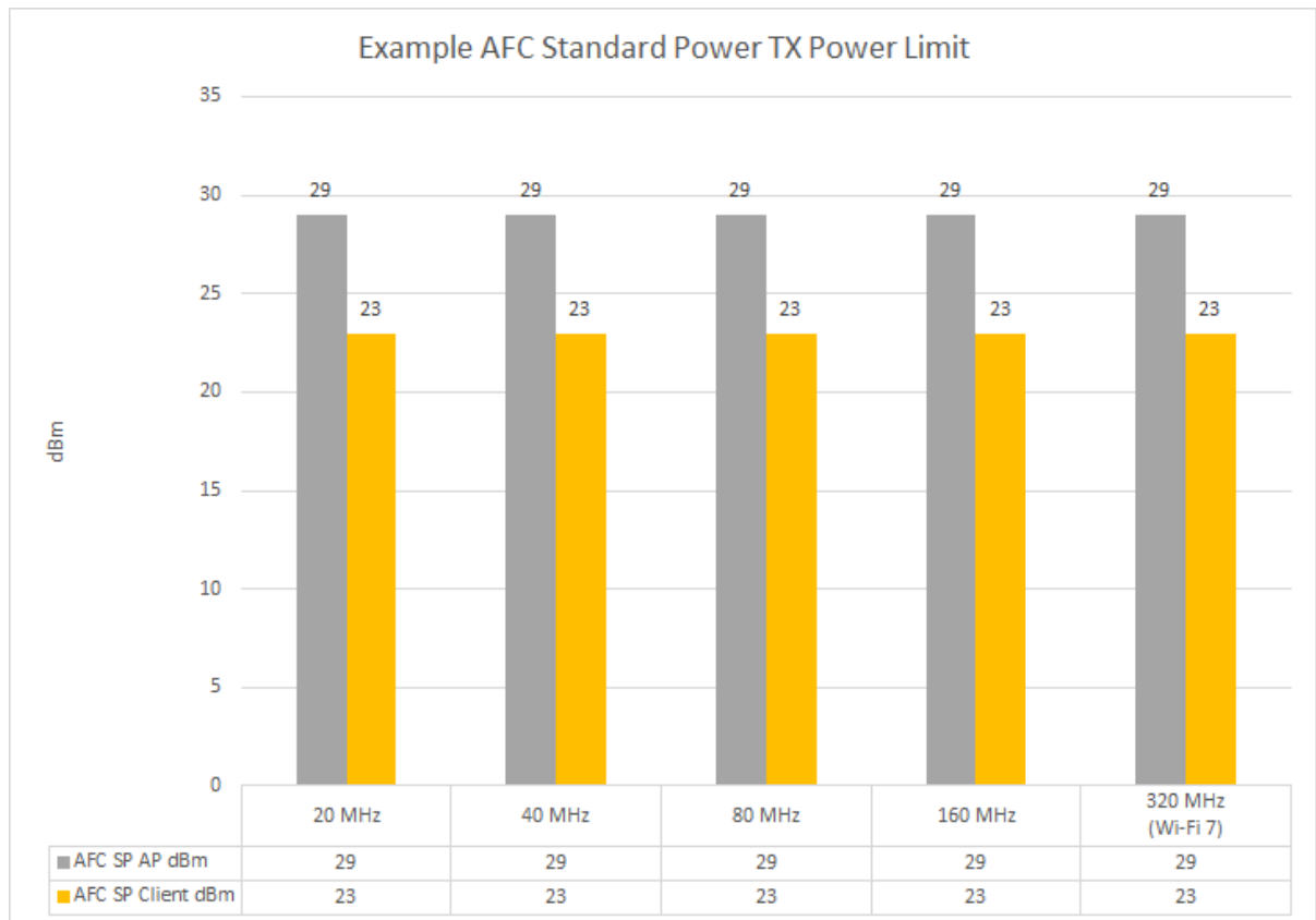
Figure 7 AFC Standard Power TX Power Limit
