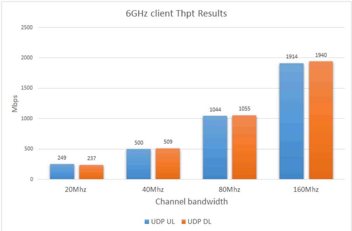
Figure 2 6GHz Throughput in Different Channel Width Settings
