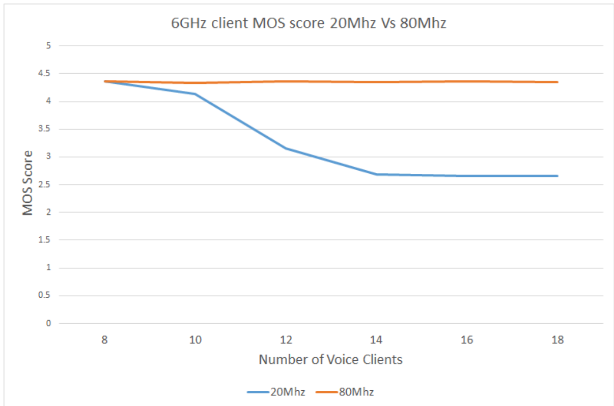
Figure 13 6GHz Client MOS Score 20MHz vs. 80MHz
