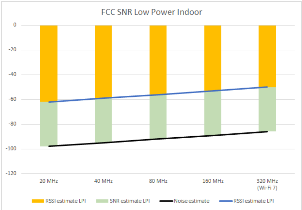
Figure 10 FCC SNR Low Power Indoor
