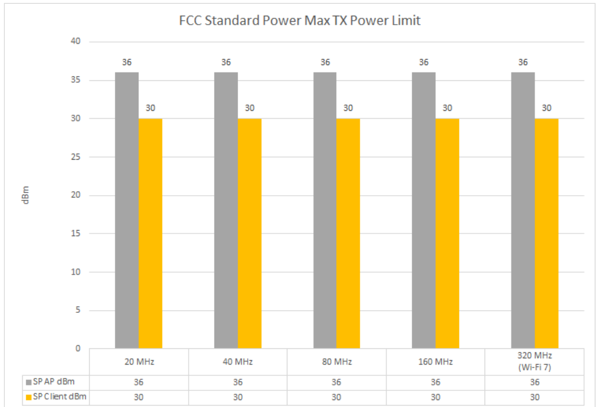
Figure 6 FCC Standard Power Max TX Power Limit
