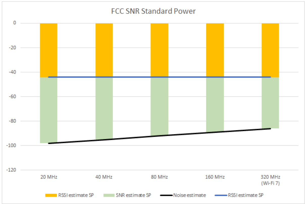
Figure 8 FCC SNR Standard Power
