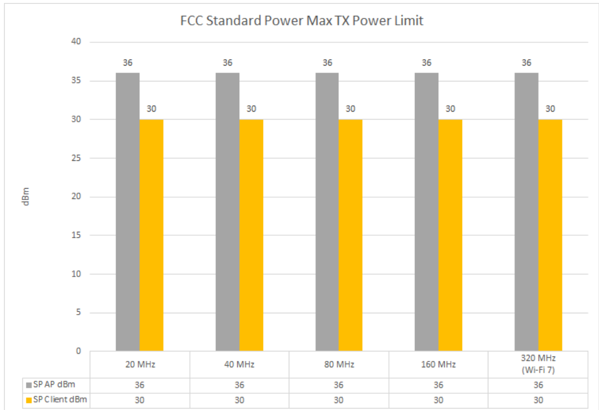
Figure 6 FCC Standard Power Max TX Power Limit
