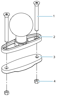
Figure 40 MT3507 Optional Mount Kits
