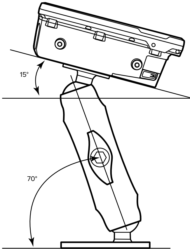
Figure 38 Orientation of Vehicle-Mount Assembly
