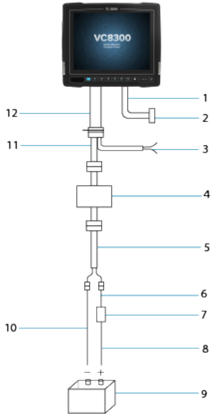
Figure 9 Connections To Vehicle DC Supply - With Power Pre-regulator For vehicles with DC power greater than 48V
