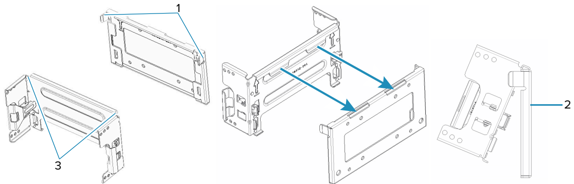
Figure 43 MT4200 Quick Release Mount Assembly
