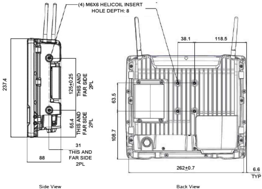
Figure 45 Drill Hole Dimensions
