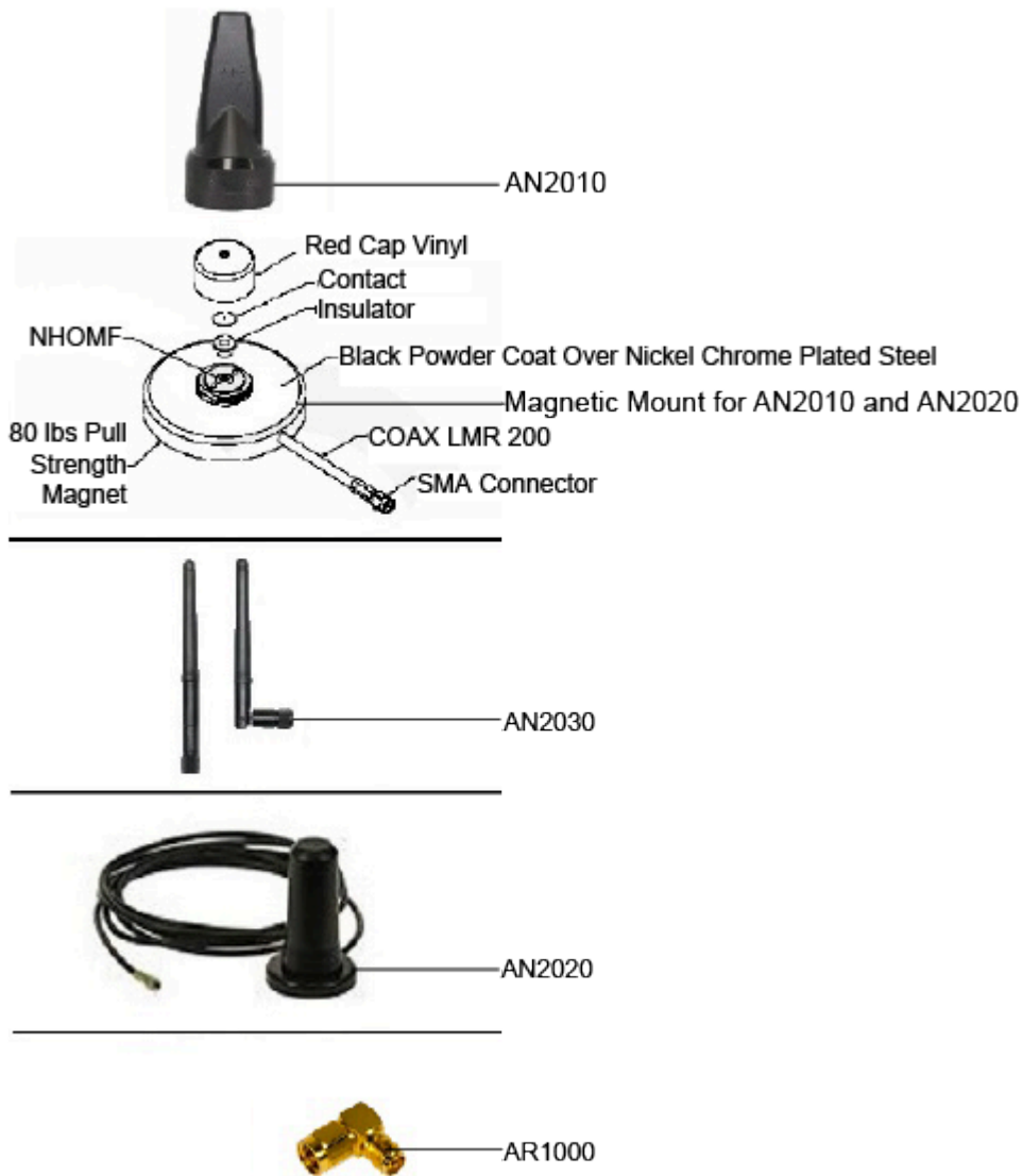
Figure 37 VC8300 Antenna Options
