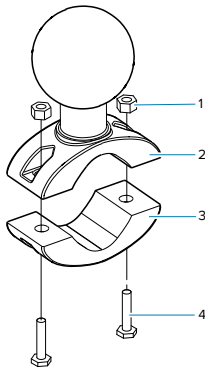
Figure 41 MT3509 Optional Mount Kit
