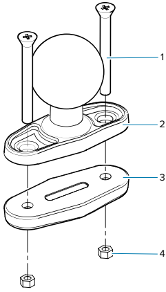
Figure 39 MT3505 Optional Mount Kits
