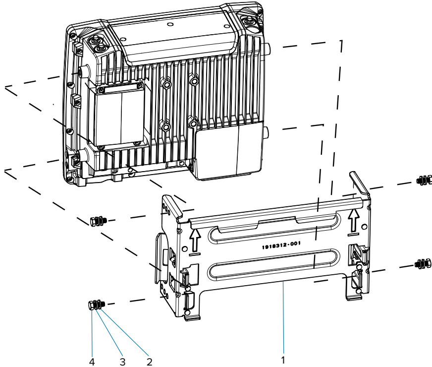
Figure 44 VC8300 and MT4200 Assembly
