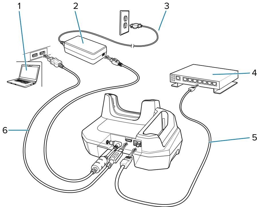
Figure 39 Setup
