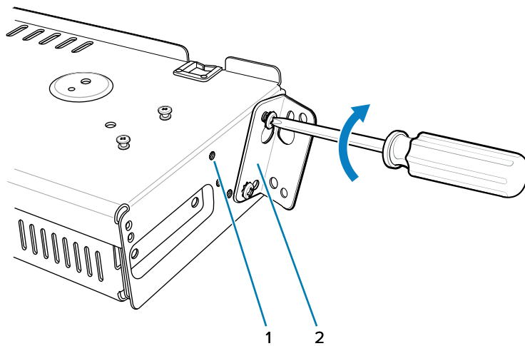
Figure 56 Flange 25° Position (4-Slot Battery Chargers)
