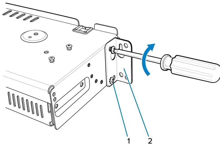
Figure 53 Flange Horizontal Position (5-Slot Cradles)
