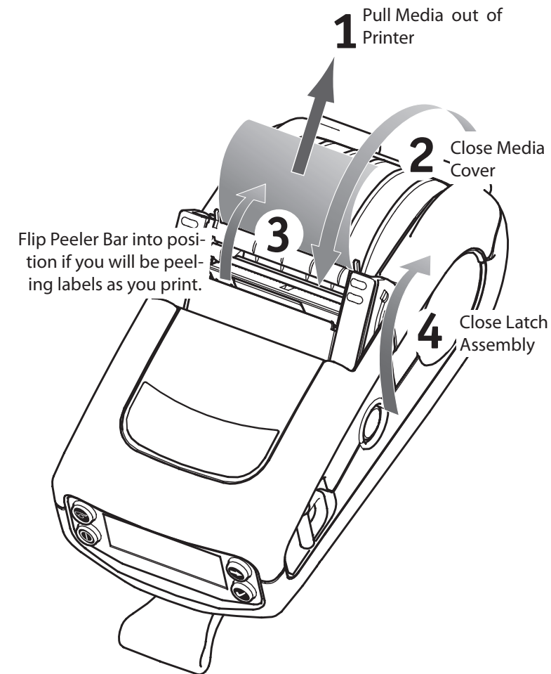
Close the Cover (common for all models)
