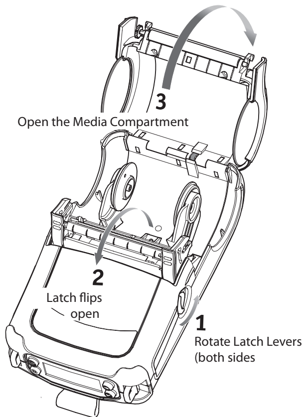
Open the QL 320
