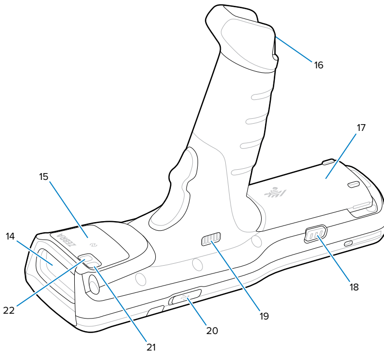
Figure 2 Bottom View
